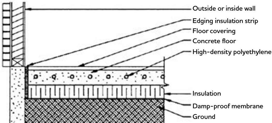
In slab heating system.
