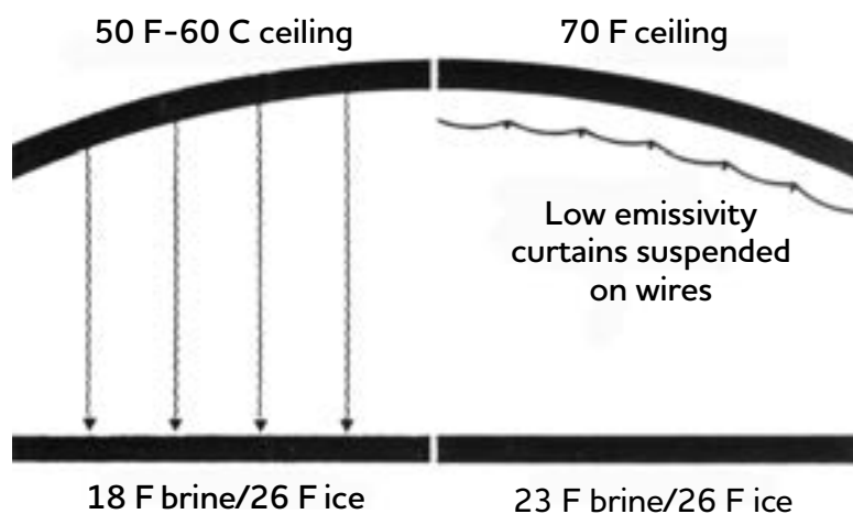
Reflective ceilings can reduce the number of light fixtures and wattage required, glare, refrigeration energy and ceiling condensation, while improving arena acoustics.
