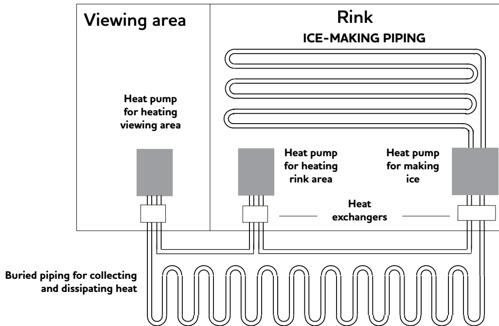
Heat pump system for a hypothetical example of a curling club.
