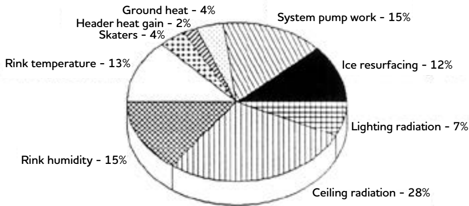
Heat loads on the refrigeration system. For a typical heated rink, radiant loads in combination with rink temperature and humidity account for almost two-thirds of the total heat gain load on the refrigeration system.
