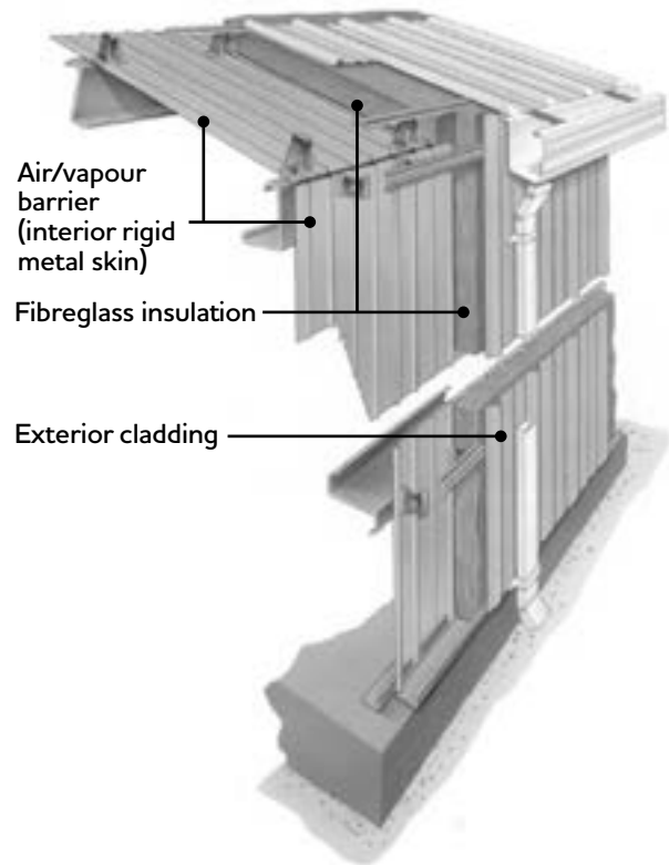
Energy efficient metal building. Standoffs between the interior metal liner and the exterior metal skin keep the insulation sandwiched in between from being compressed. The metal liner also serves as an air/vapour barrier.
