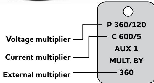
Front panel of an electronic meter for reading energy and demand. The meter is shown in energy consumed mode (left) and in demand mode (right). The tag below gives the multipliers for this meter.
