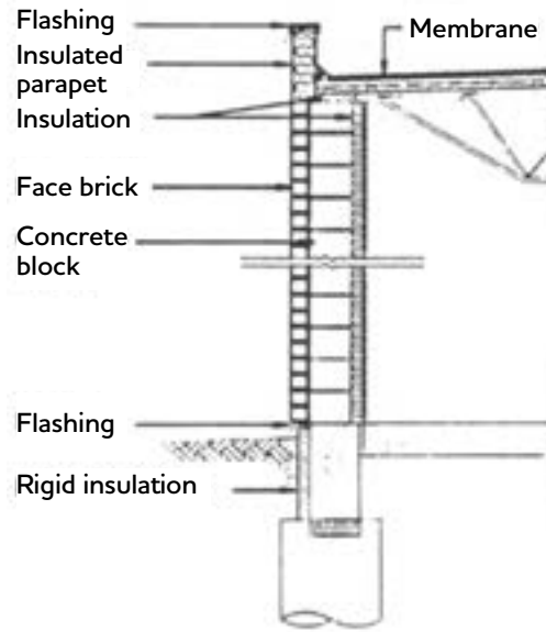
Typical brick and block wall construction.
