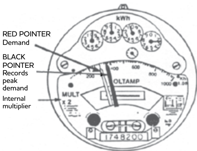
Typical electrical demand meter. The red pointer tracks demand, while the black pointer tracks peak demand.
