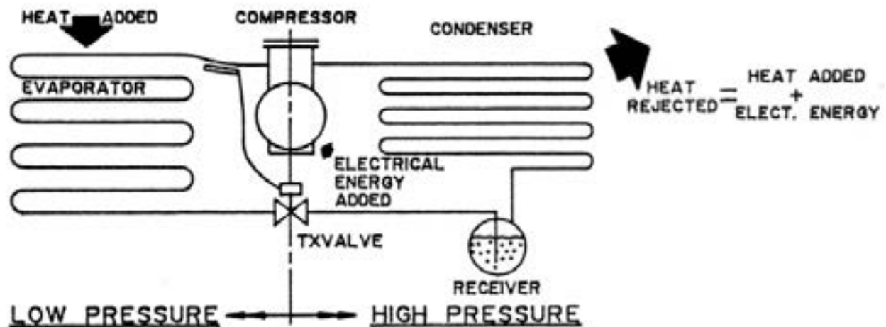
Refrigeration cycle
