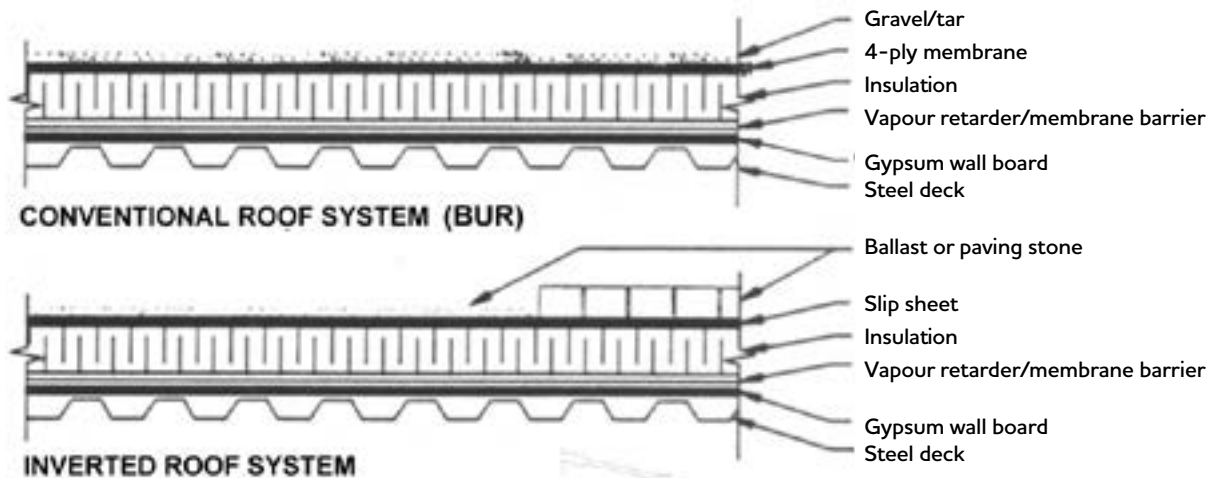
Conventional built-up and inverted "flat" roof systems.
